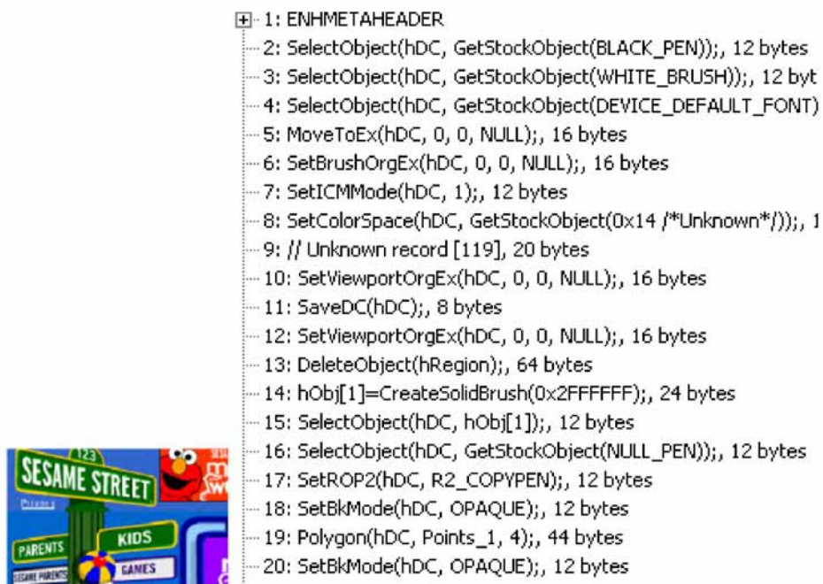
Fig. 1. Realization of an Enhanced Metafile (EMF) and representative EMF commands.
